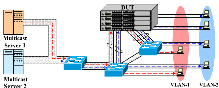
Figure 1. An Example of a Virtual Bridged LAN Test Topology
